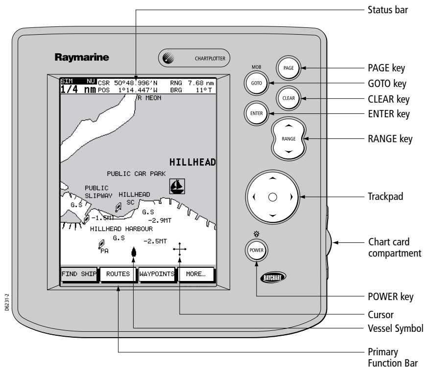
Figure 1-1: RC435/435i Chartplotter Operating Controls
