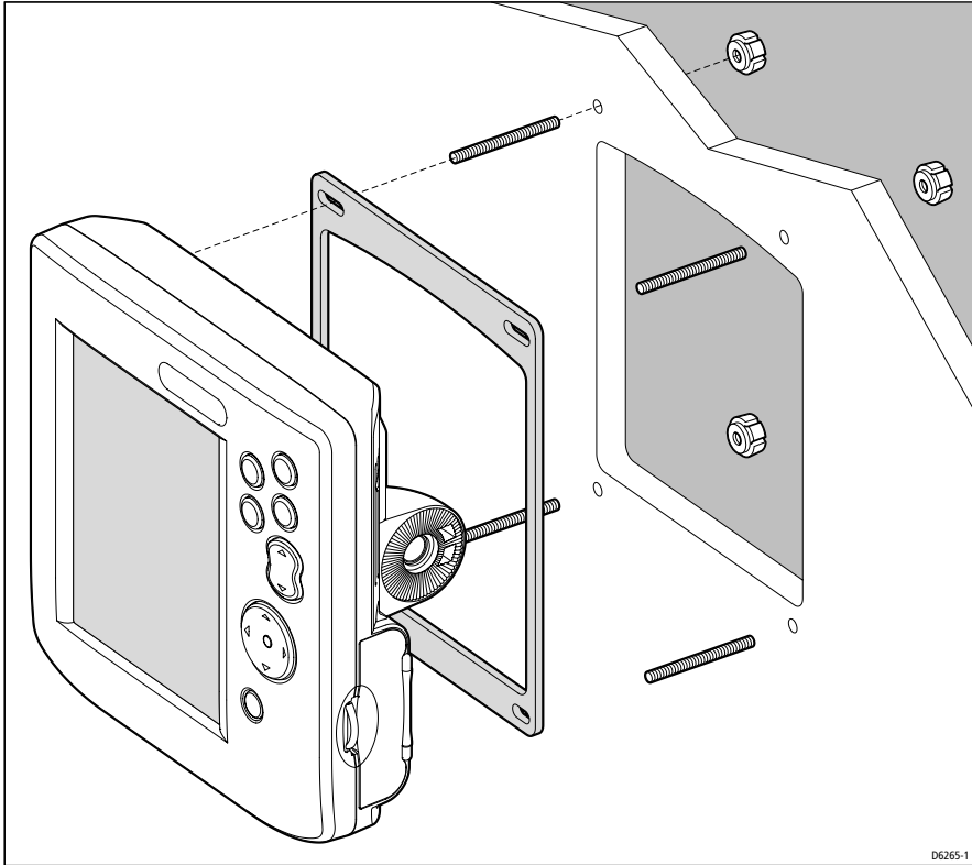
Figure 2-3: RC435(i) Panel Mounting Arrangement
